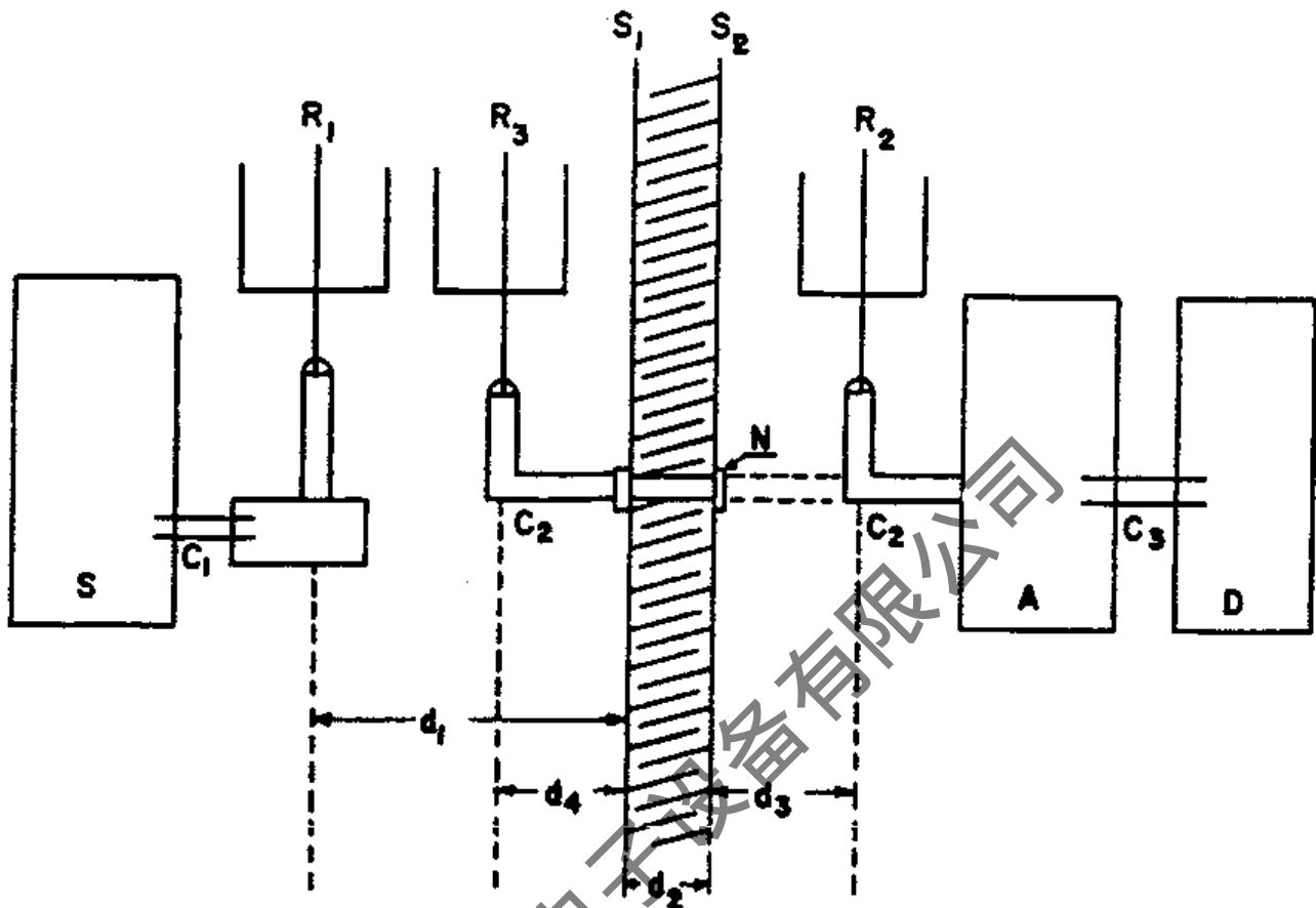
FIGURE 5.—Attenuation test for plane waves (wave impedance = 577 ohms).
